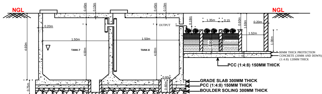
SECTION AT "BB"
